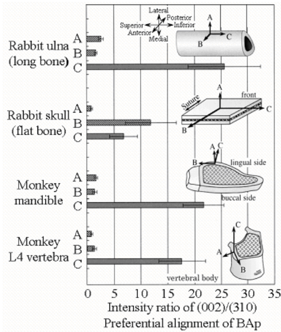
Fig. 1 Preferential alignment of the BAp c-axis in typical mature intact cortical bones.
